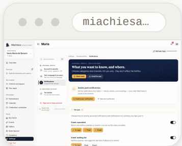
Fig. 1 The page separates device push status from profile preferences.
